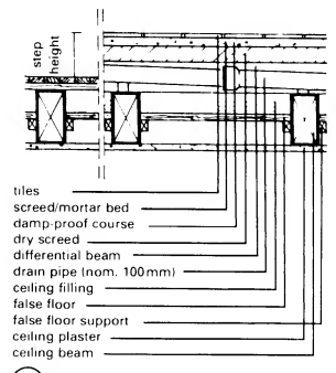
⑪ Laying waste pipe below new floor
